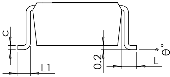
Side View 1
